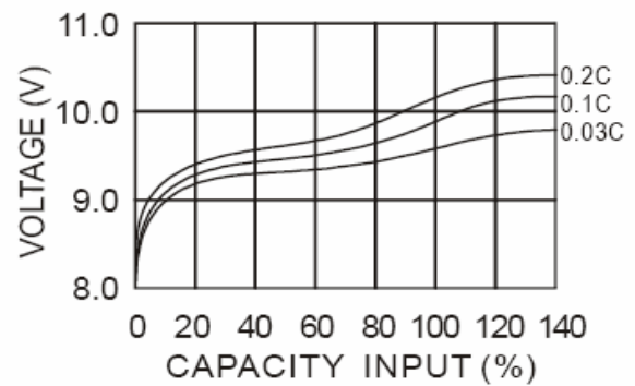
TYPICAL CHARGE CURVE
