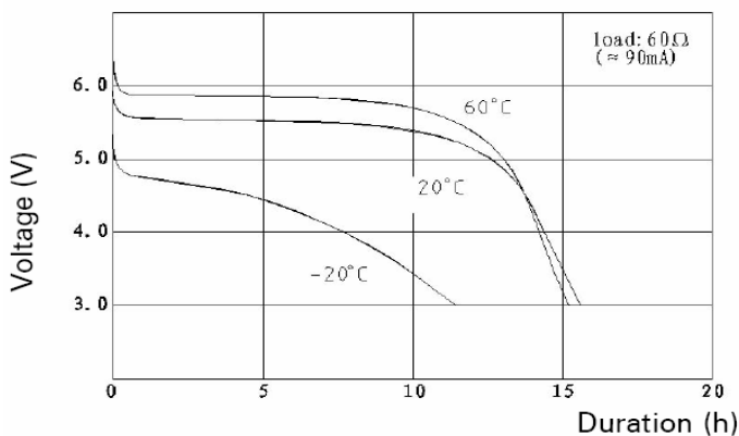
Temperature characteristics
