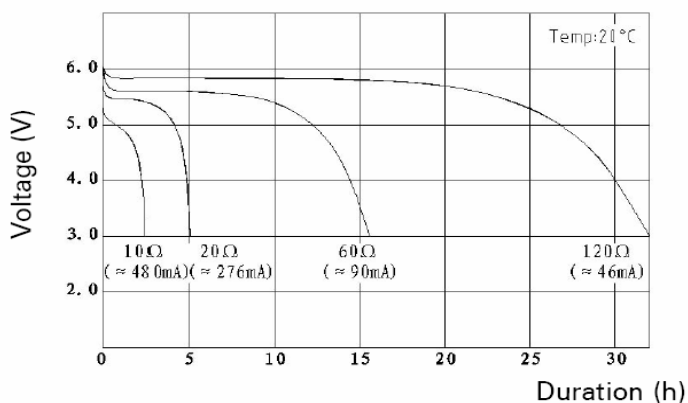
Typical discharge characteristics
