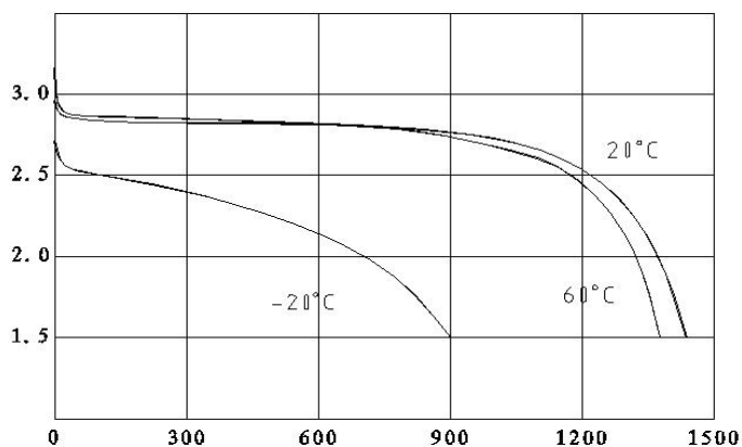
temperature characteristics(100mAh)
